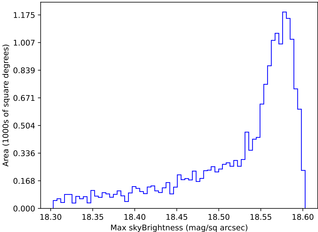
weather_cloudso8v3.4_10yrs WFD y band: Max skyBrightness
