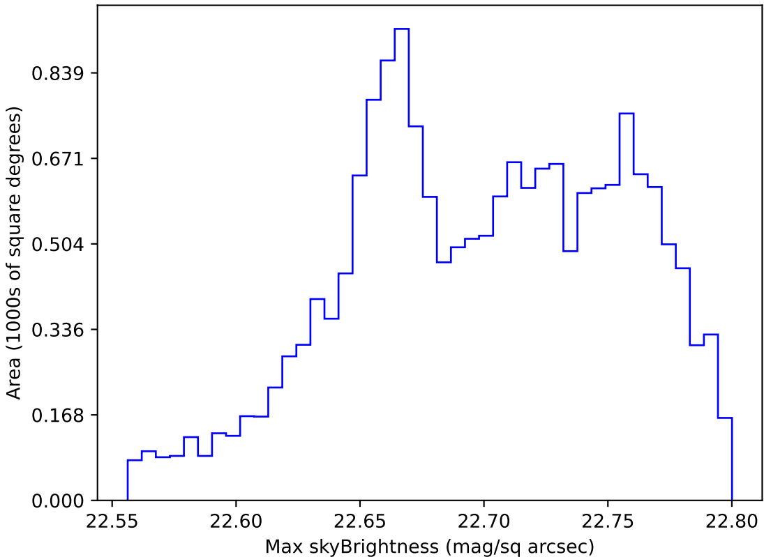
weather_cloudso8v3.4_10yrs WFD u band: Max skyBrightness
