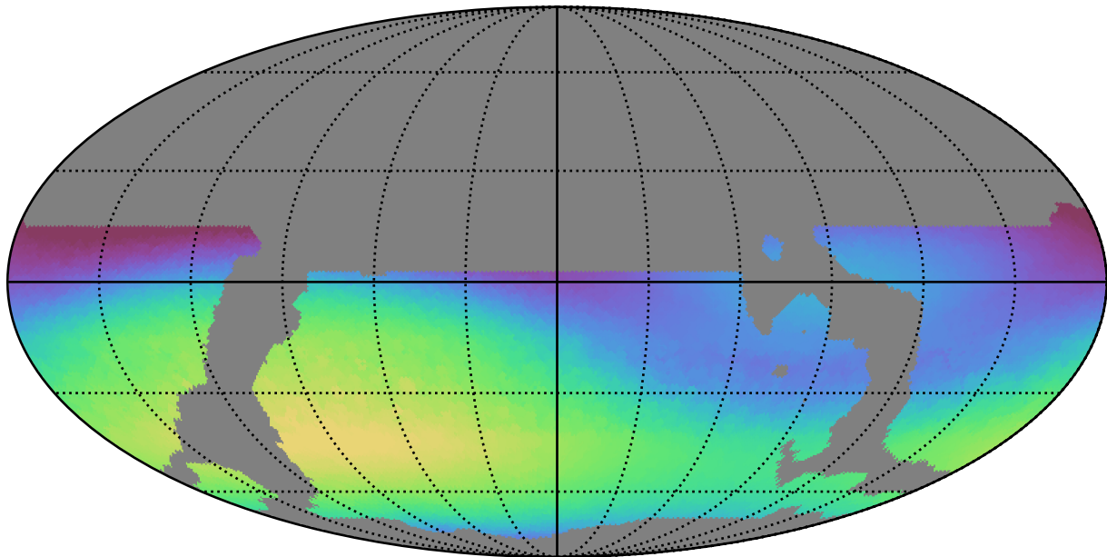
weather_cloudso8v3.4_10yrs WFD r band: Max skyBrightness
