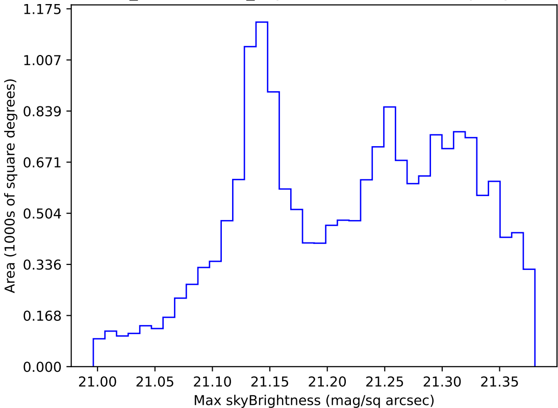
weather_cloudso8v3.4_10yrs WFD r band: Max skyBrightness
