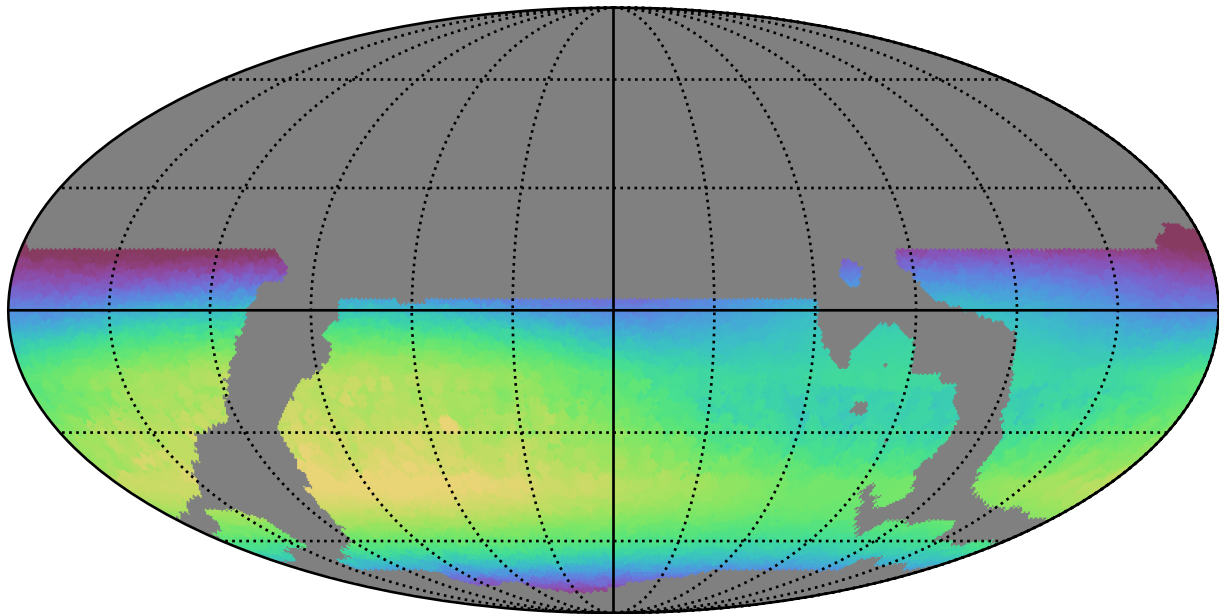
weather_cloudso8v3.4_10yrs WFD i band: Max skyBrightness
