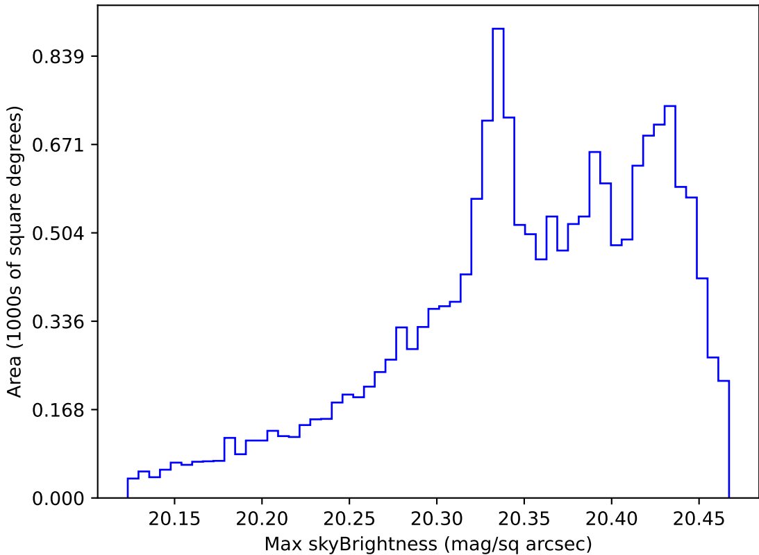
weather_cloudso8v3.4_10yrs WFD i band: Max skyBrightness
