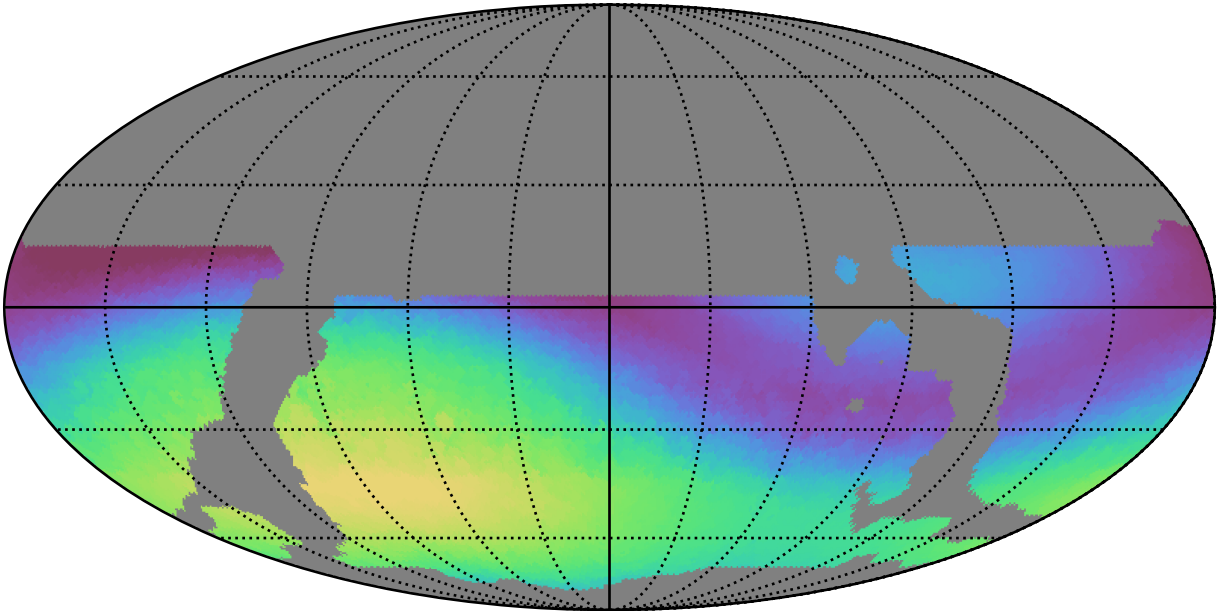
weather_cloudso8v3.4_10yrs WFD g band: Max skyBrightness
