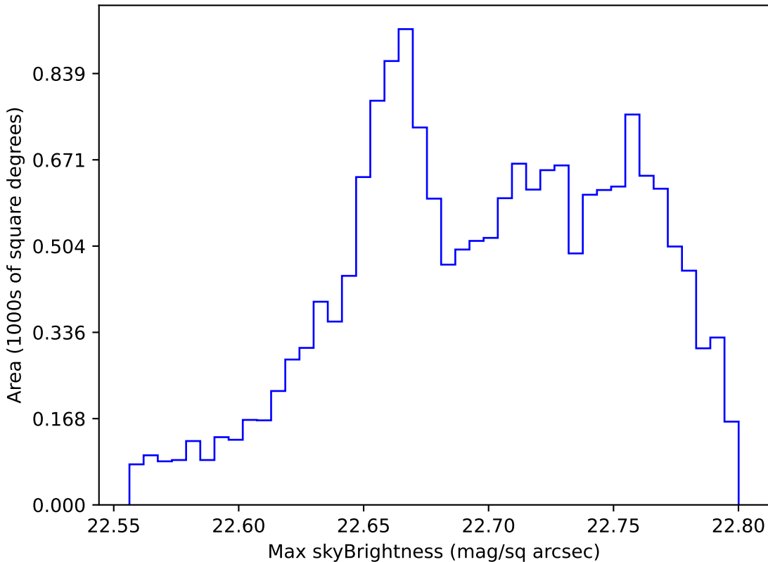
weather_cloudso8v3.4_10yrs WFD all bands: Max skyBrightness
