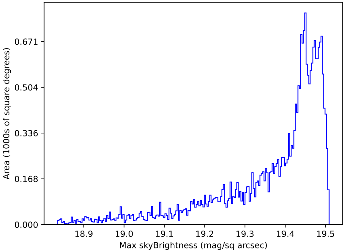
weather_cloudso8v3.4_10yrs All sky z band: Max skyBrightness
