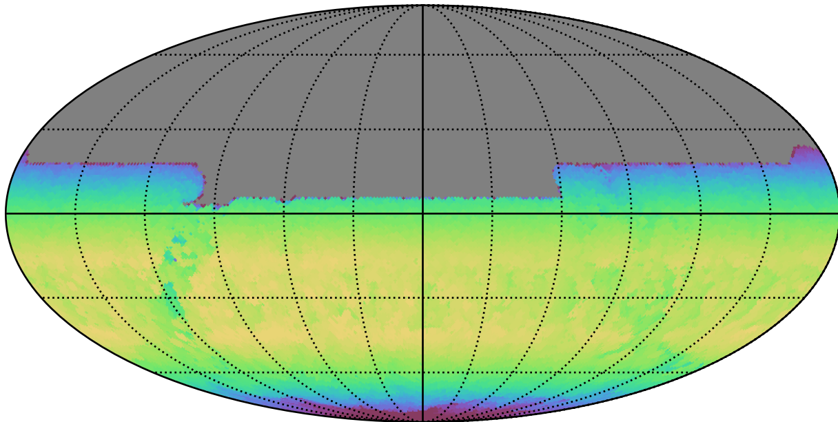
weather_cloudso8v3.4_10yrs All sky y band: Max skyBrightness
