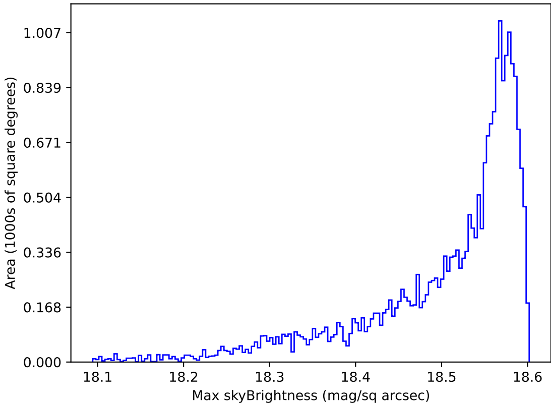
weather_cloudso8v3.4_10yrs All sky y band: Max skyBrightness
