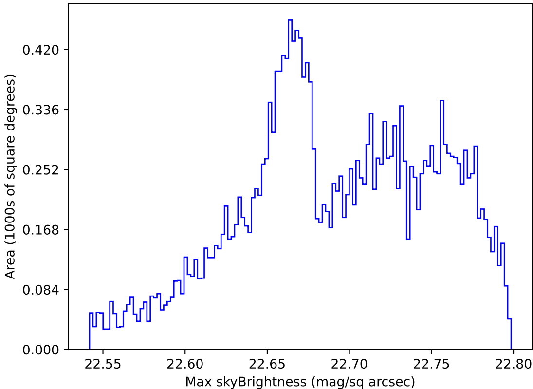
weather_cloudso8v3.4_10yrs All sky u band: Max skyBrightness
