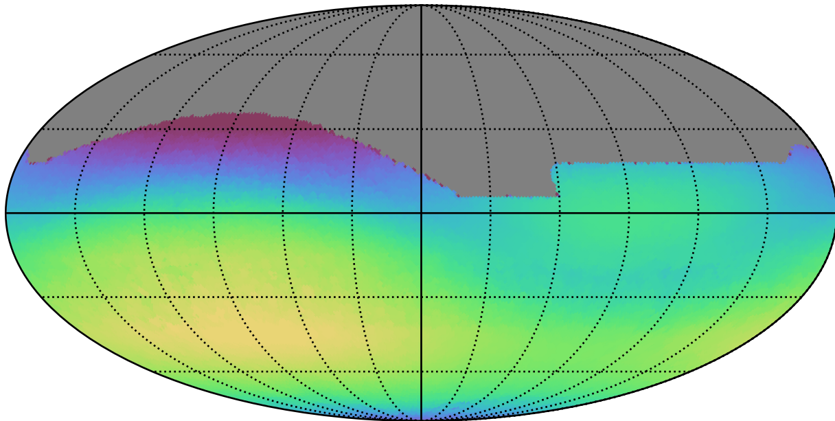
weather_cloudso8v3.4_10yrs All sky r band: Max skyBrightness
