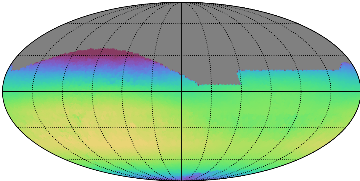
weather_cloudso8v3.4_10yrs All sky i band: Max skyBrightness
