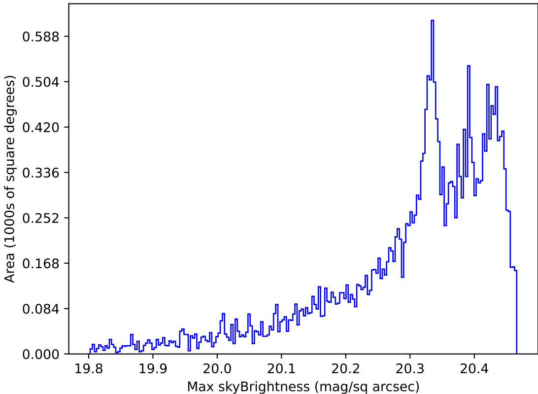
weather_cloudso8v3.4_10yrs All sky i band: Max skyBrightness
