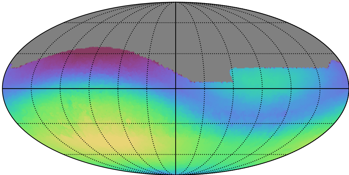
weather_cloudso8v3.4_10yrs All sky g band: Max skyBrightness
