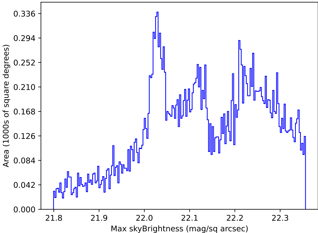
weather_cloudso8v3.4_10yrs All sky g band: Max skyBrightness
