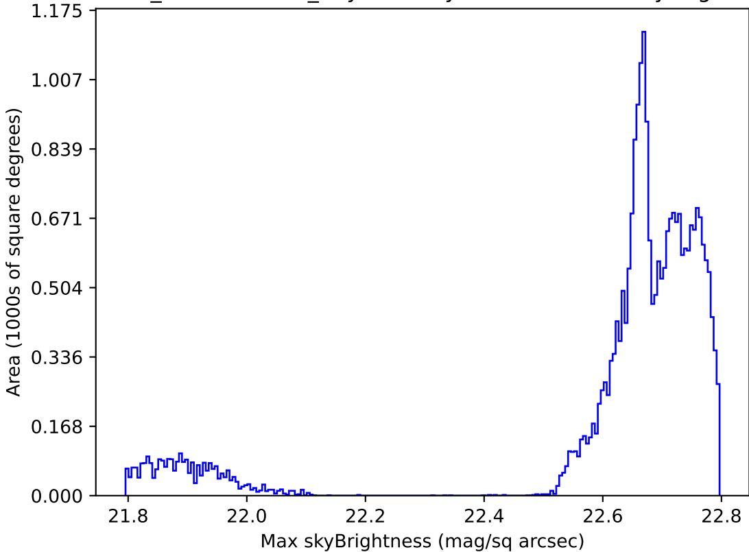
weather_cloudso8v3.4_10yrs All sky all bands: Max skyBrightness
