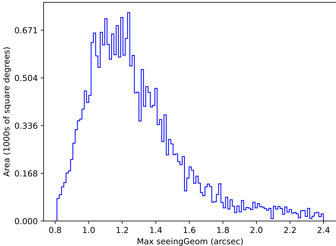
weather_cloudso8v3.4_10yrs Yr 1 z band: Max seeingGeom
