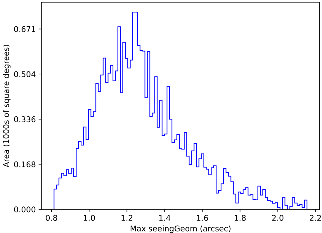
weather_cloudso8v3.4_10yrs Yr 1 y band: Max seeingGeom
