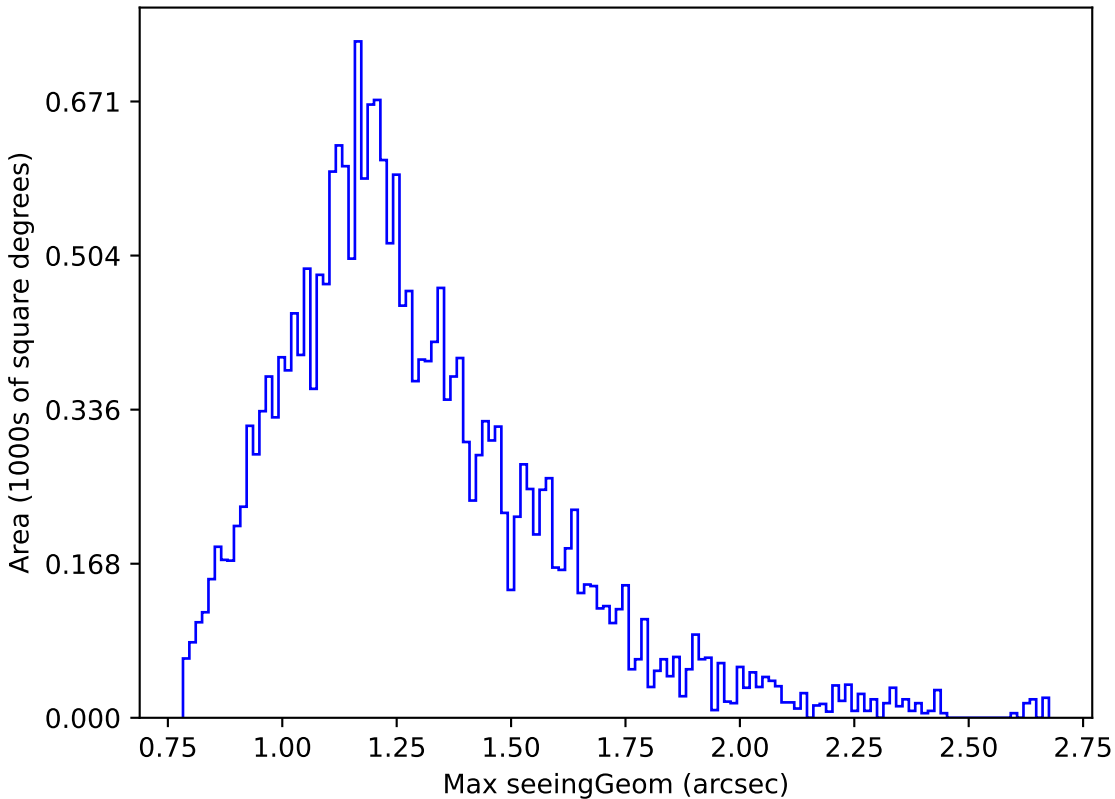
weather_cloudso8v3.4_10yrs Yr 1 u band: Max seeingGeom
