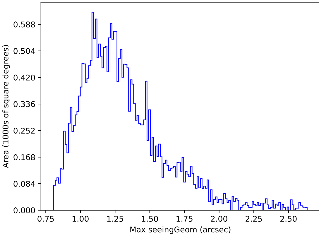
weather_cloudso8v3.4_10yrs Yr 1 i band: Max seeingGeom
