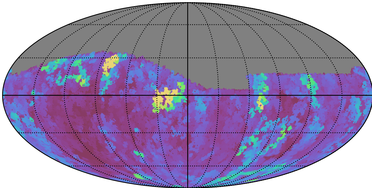
weather_cloudso8v3.4_10yrs Yr 1 g band: Max seeingGeom
