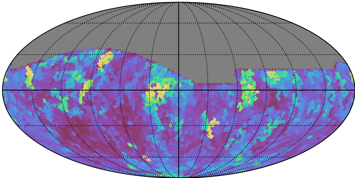
weather_cloudso8v3.4_10yrs Yr 1 all bands: Max seeingGeom
