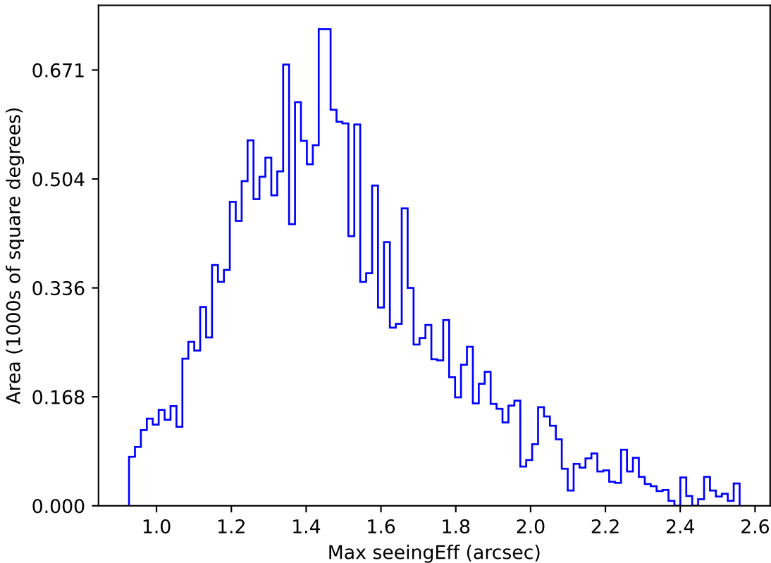
weather_cloudso8v3.4_10yrs Yr 1 y band: Max seeingEff
