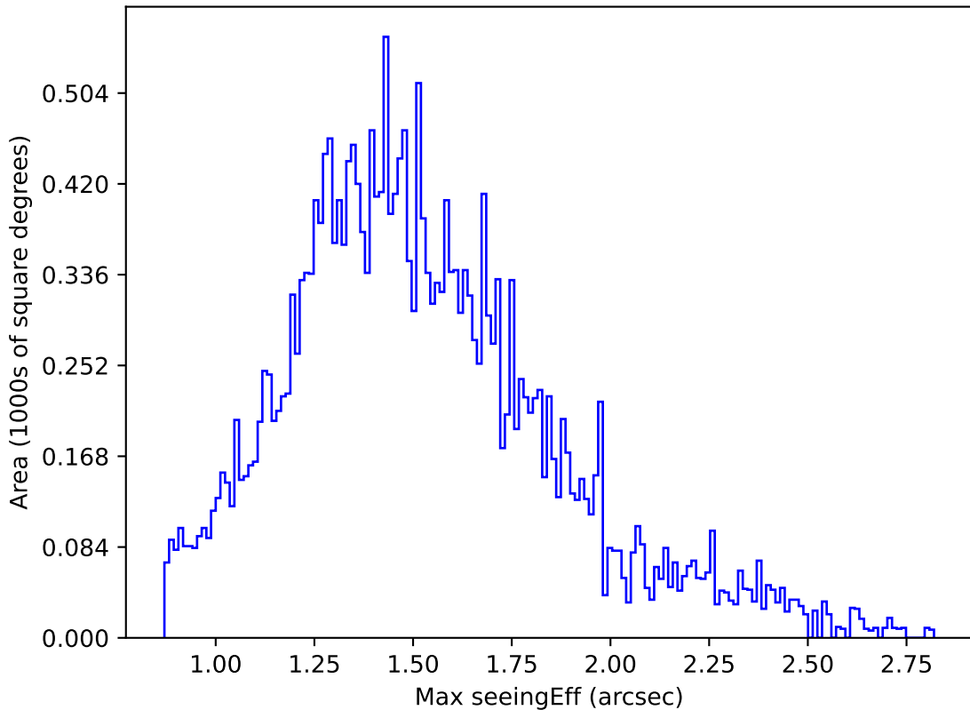
weather_cloudso8v3.4_10yrs Yr 1 r band: Max seeingEff
