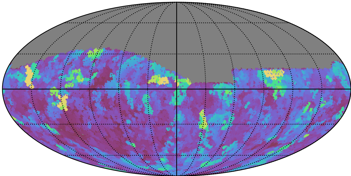
weather_cloudso8v3.4_10yrs Yr 1 i band: Max seeingEff
