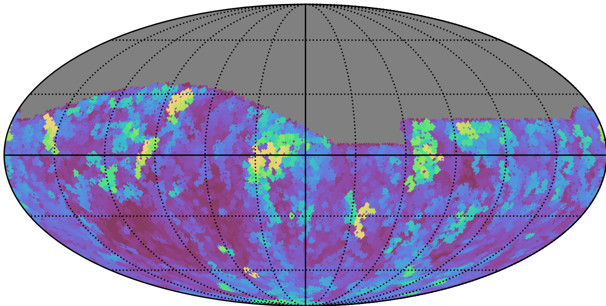
weather_cloudso8v3.4_10yrs Yr 1 all bands: Max seeingEff
