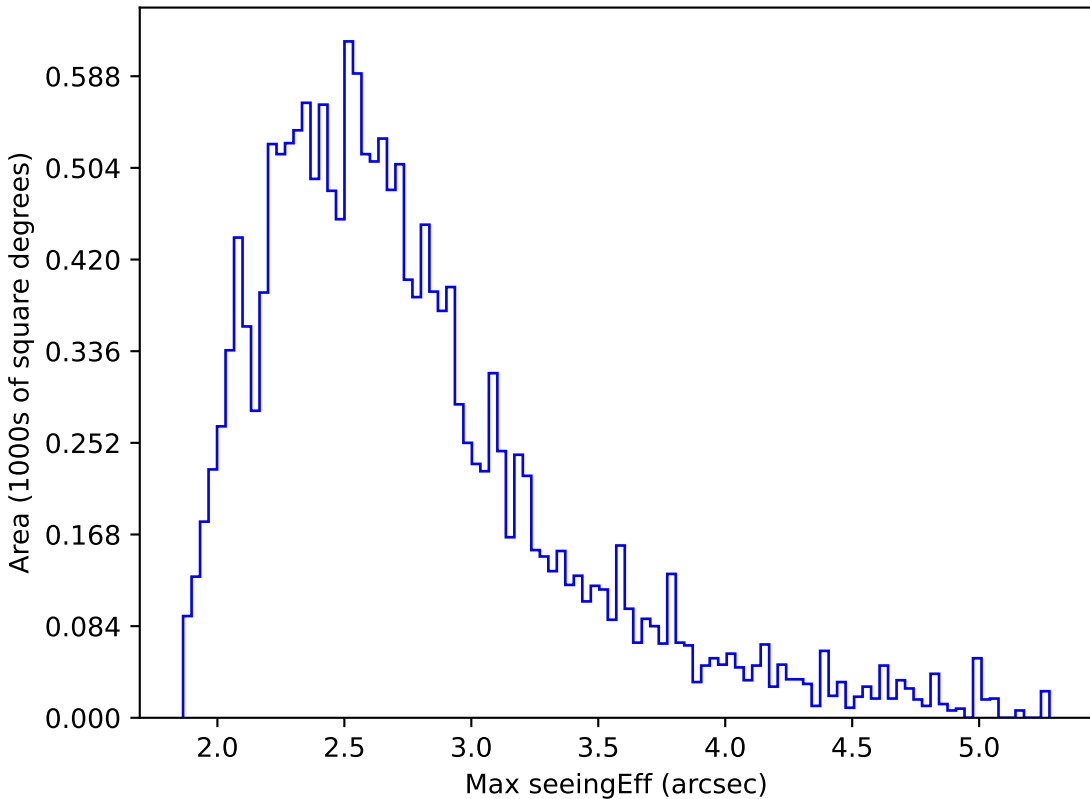
weather_cloudso8v3.4_10yrs WFD z band: Max seeingEff
