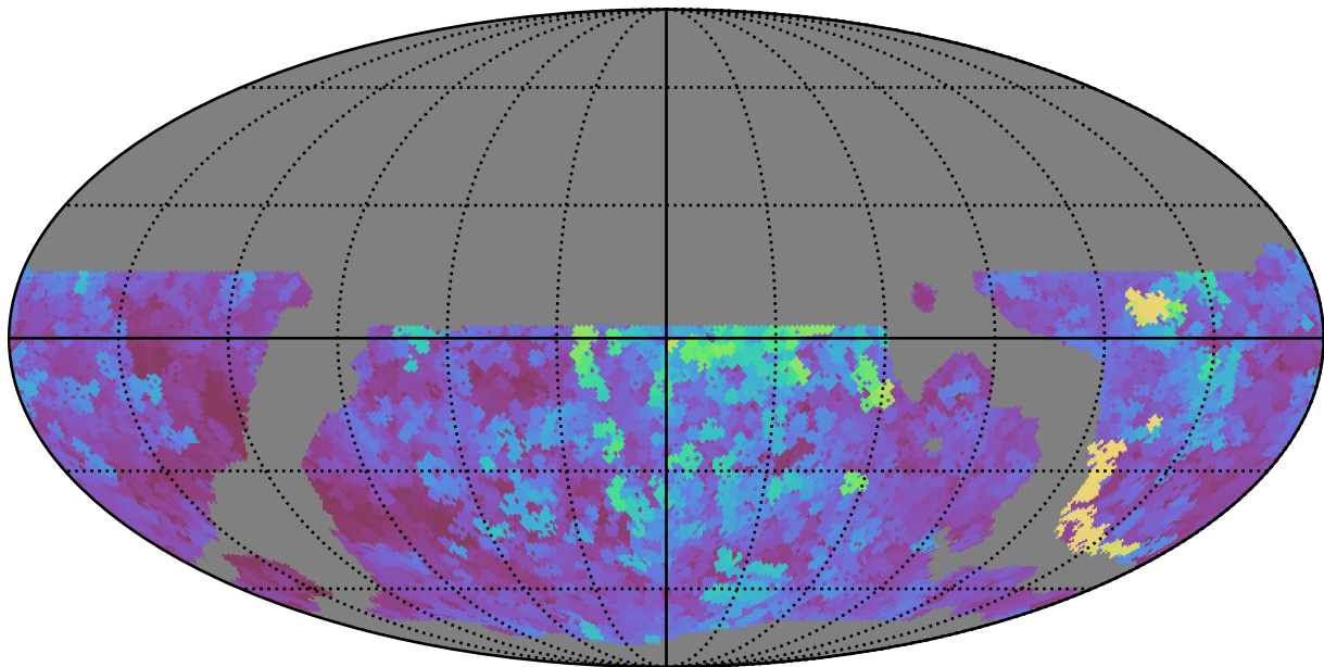
weather_cloudso8v3.4_10yrs WFD y band: Max seeingEff
