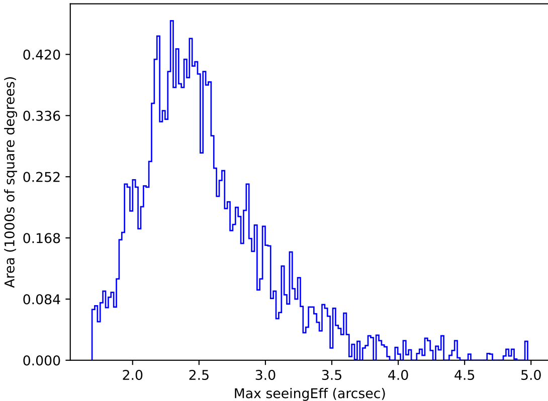
weather_cloudso8v3.4_10yrs WFD y band: Max seeingEff
