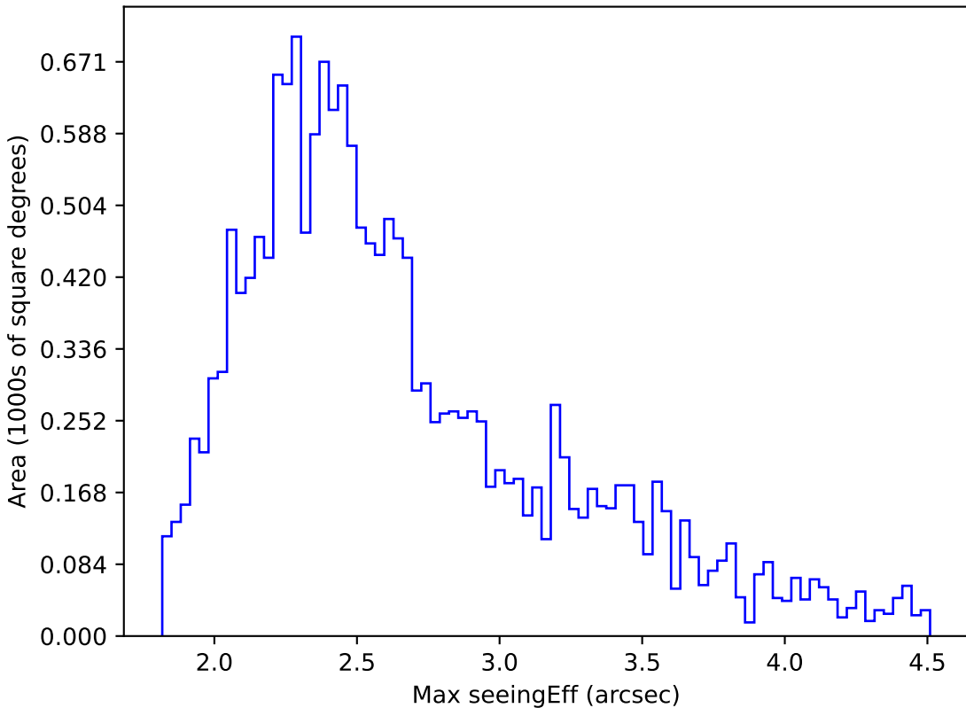
weather_cloudso8v3.4_10yrs WFD u band: Max seeingEff
