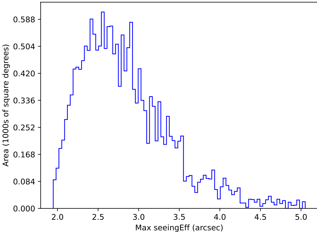
weather_cloudso8v3.4_10yrs WFD r band: Max seeingEff
