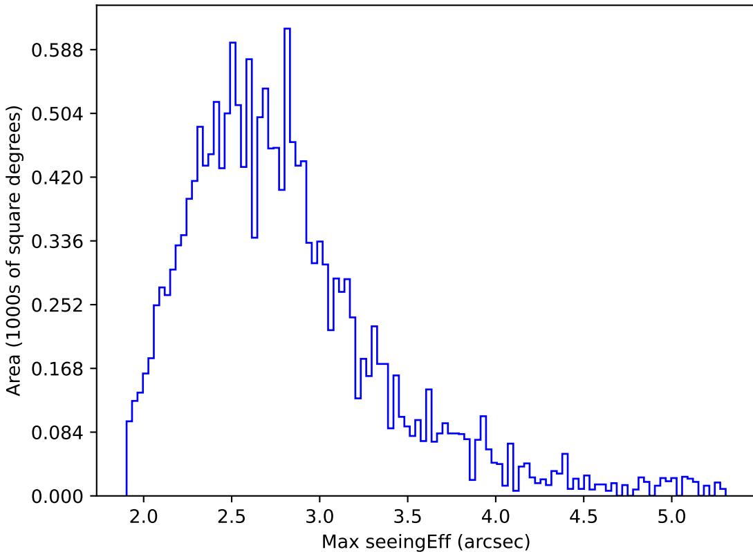
weather_cloudso8v3.4_10yrs WFD i band: Max seeingEff
