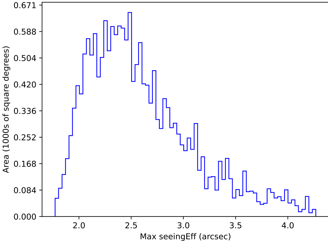
weather_cloudso8v3.4_10yrs WFD g band: Max seeingEff
