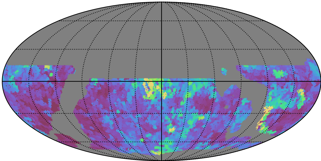
weather_cloudso8v3.4_10yrs WFD all bands: Max seeingEff
