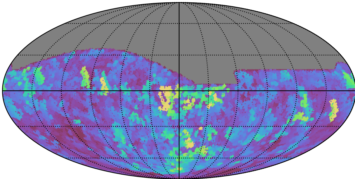
weather_cloudso8v3.4_10yrs All sky z band: Max seeingEff
