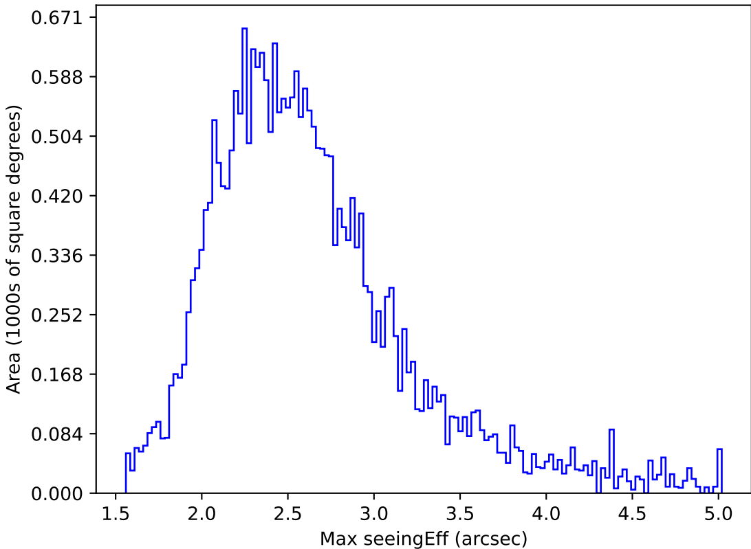
weather_cloudso8v3.4_10yrs All sky z band: Max seeingEff
