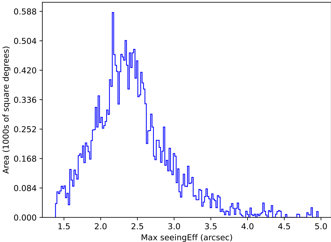
weather_cloudso8v3.4_10yrs All sky y band: Max seeingEff
