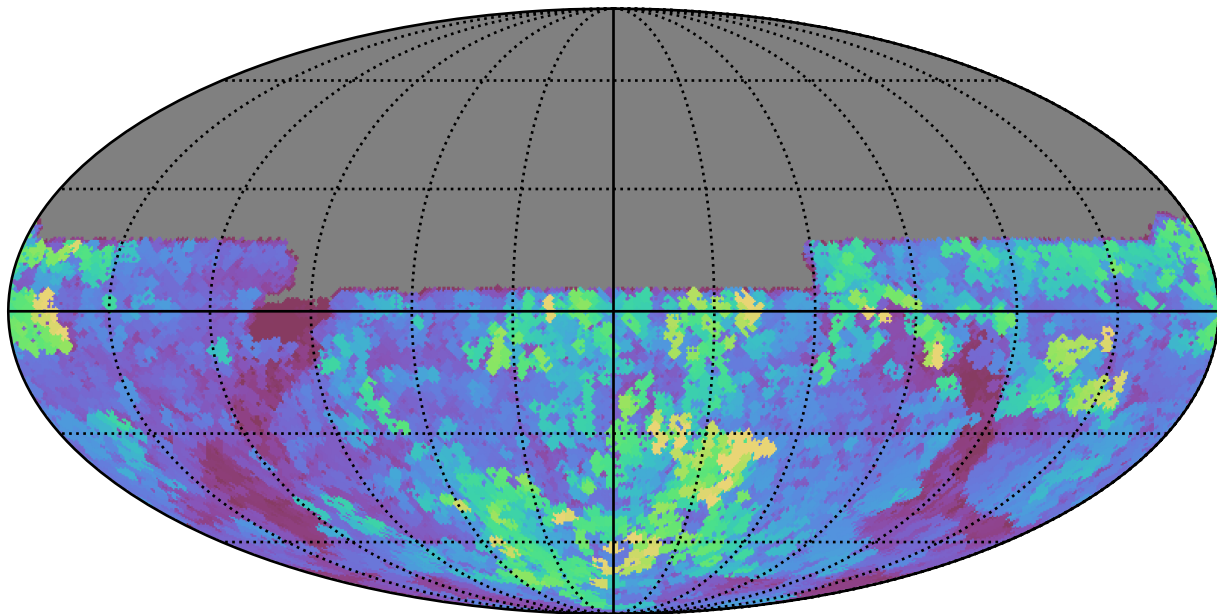
weather_cloudso8v3.4_10yrs All sky u band: Max seeingEff
