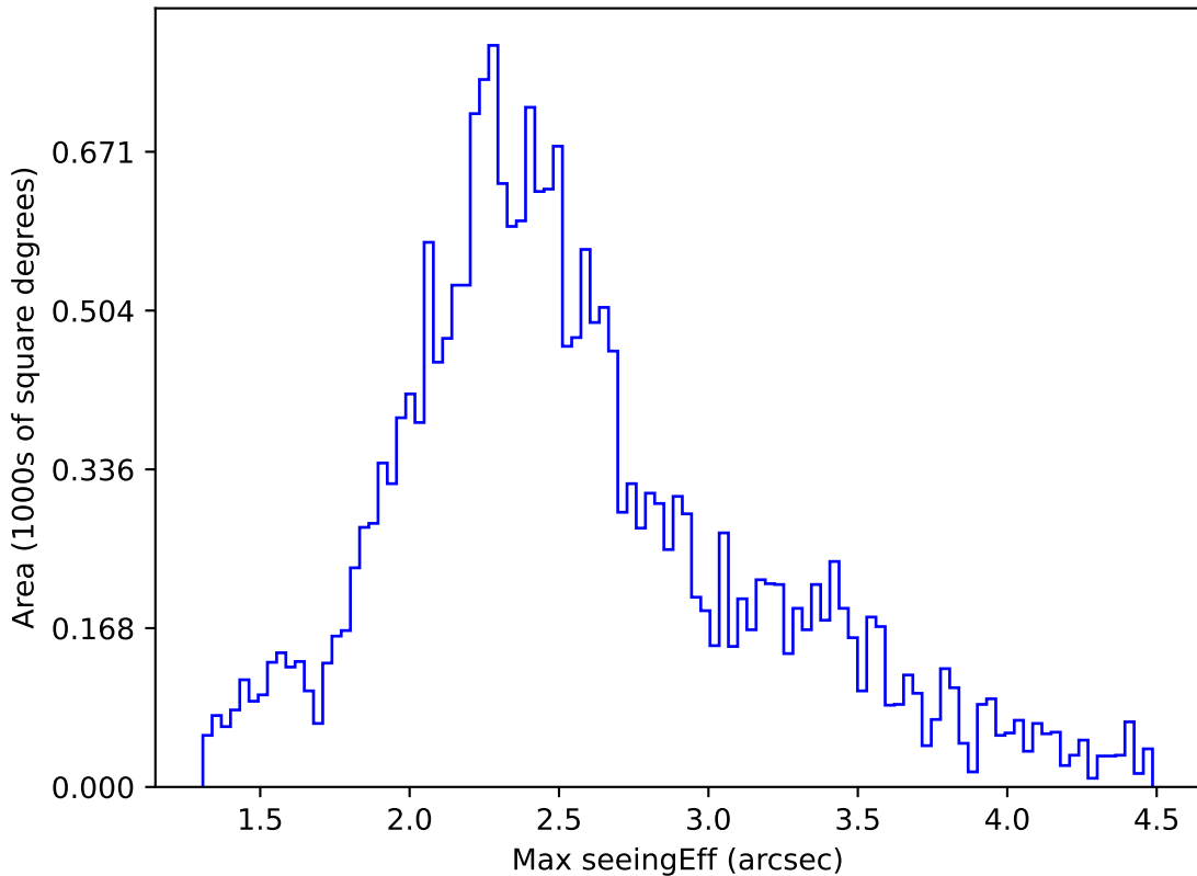
weather_cloudso8v3.4_10yrs All sky u band: Max seeingEff
