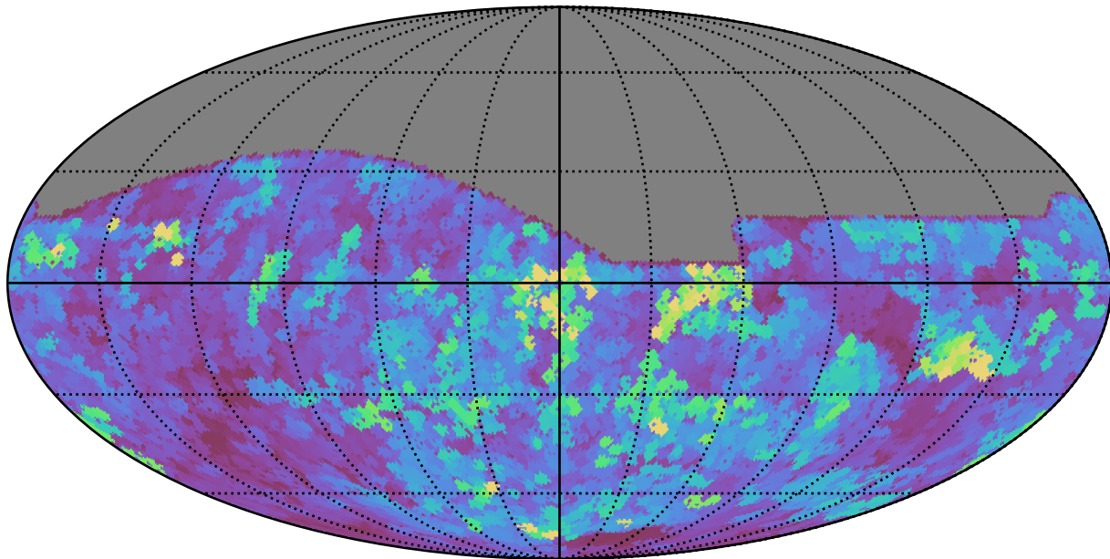
weather_cloudso8v3.4_10yrs All sky r band: Max seeingEff
