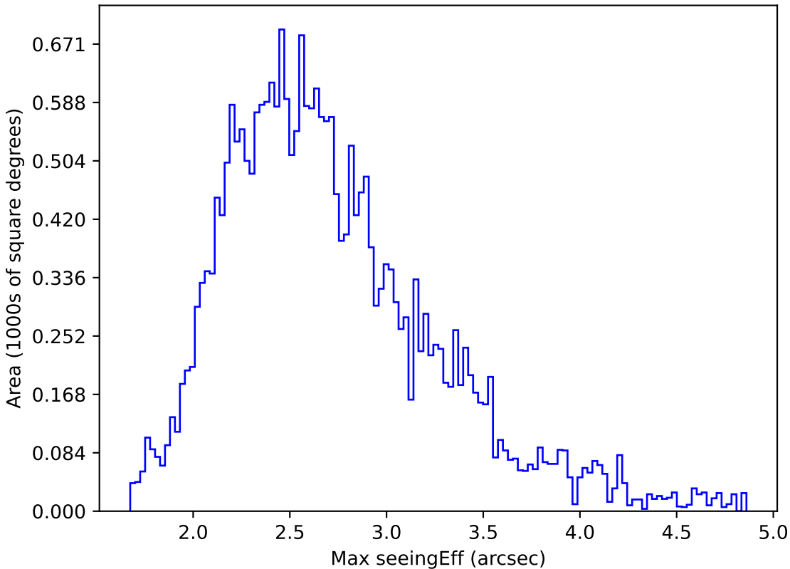
weather_cloudso8v3.4_10yrs All sky r band: Max seeingEff
