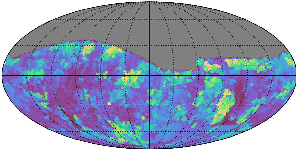
weather_cloudso8v3.4_10yrs All sky g band: Max seeingEff
