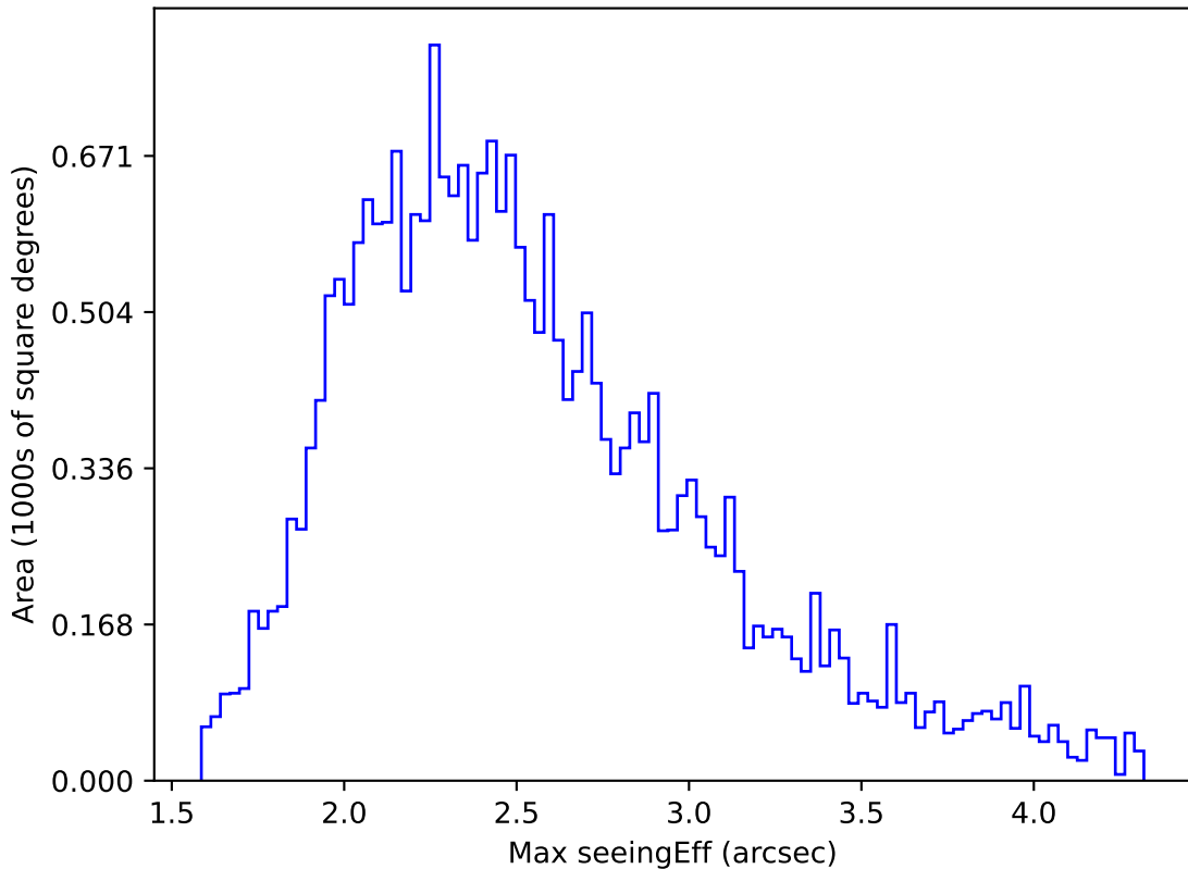
weather_cloudso8v3.4_10yrs All sky g band: Max seeingEff
