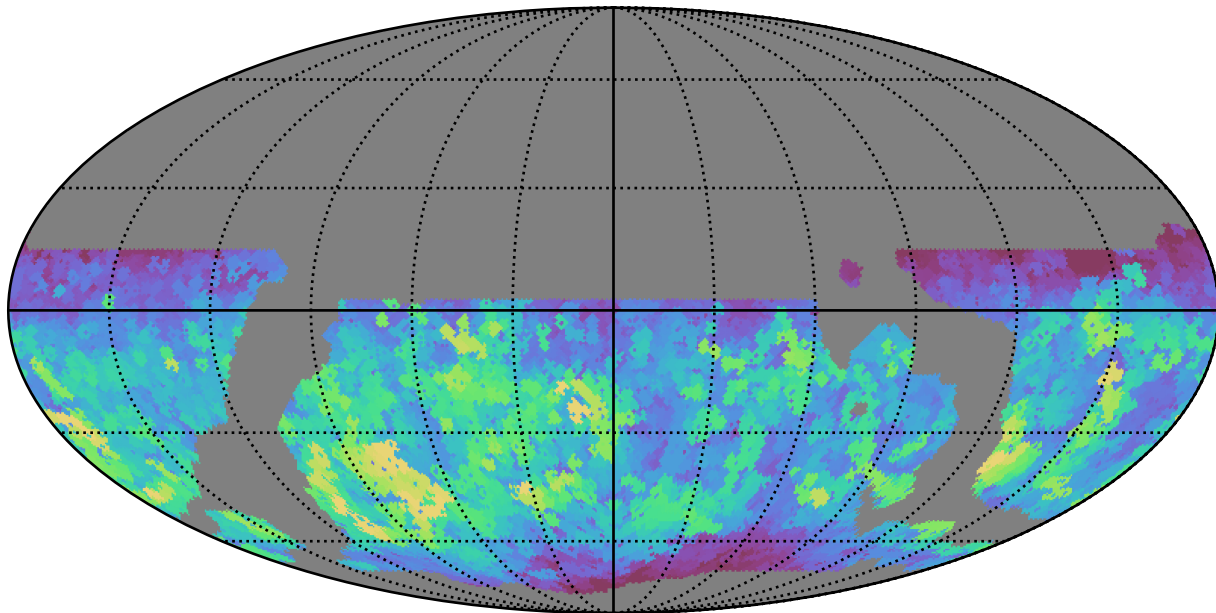
weather_cloudso8v3.4_10yrs WFD all bands: Max saturation_mag
