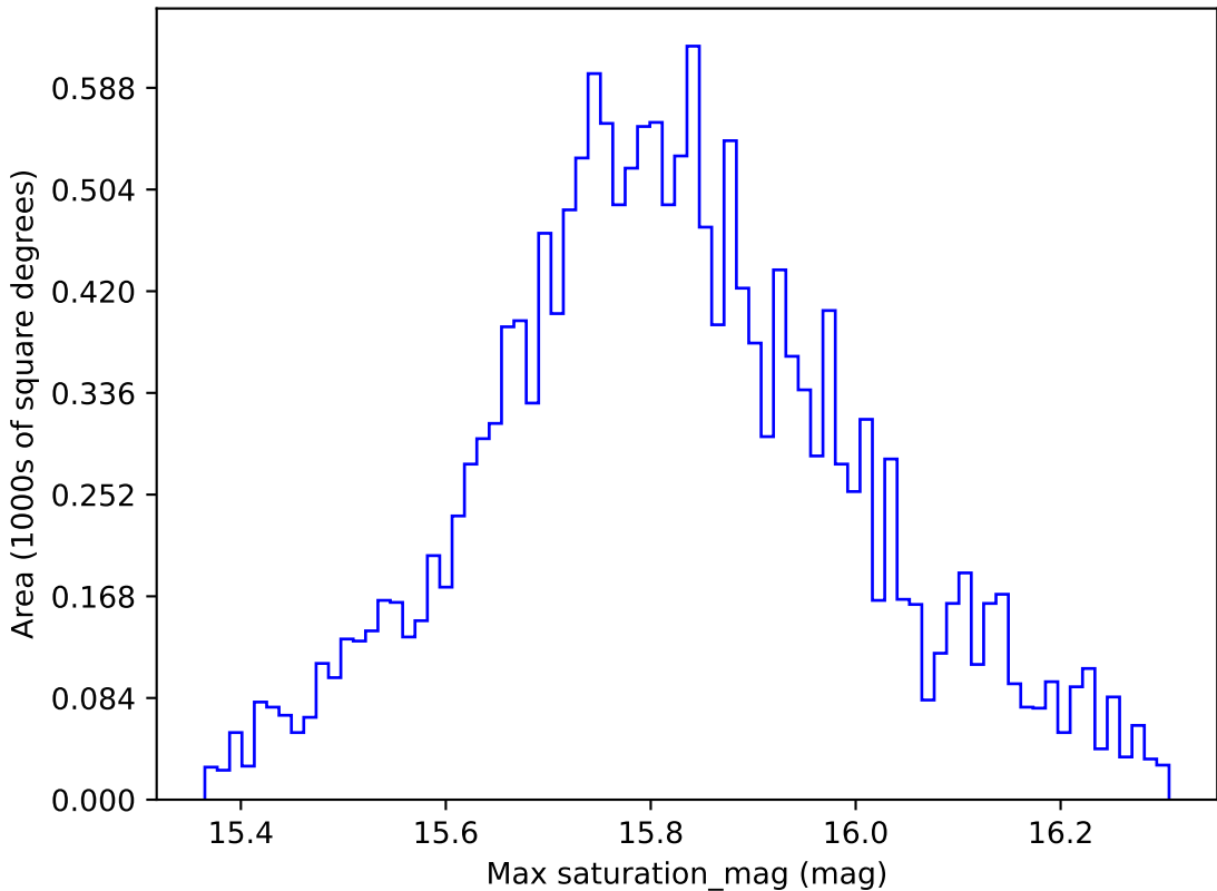
weather_cloudso8v3.4_10yrs WFD all bands: Max saturation_mag
