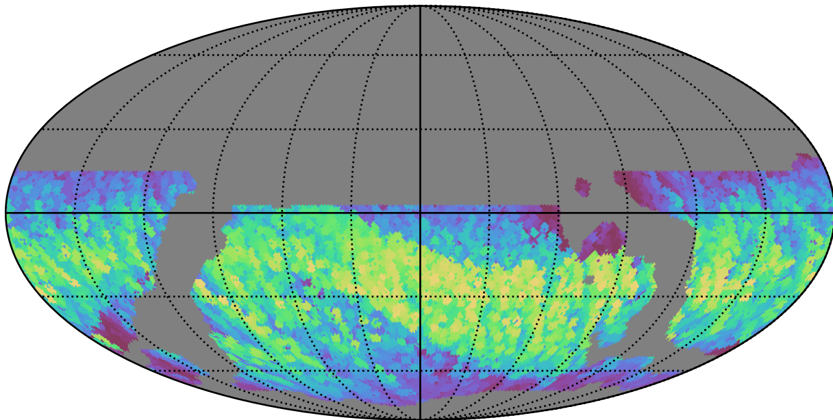
weather_cloudso8v3.4_10yrs WFD z band: Max normairmass
