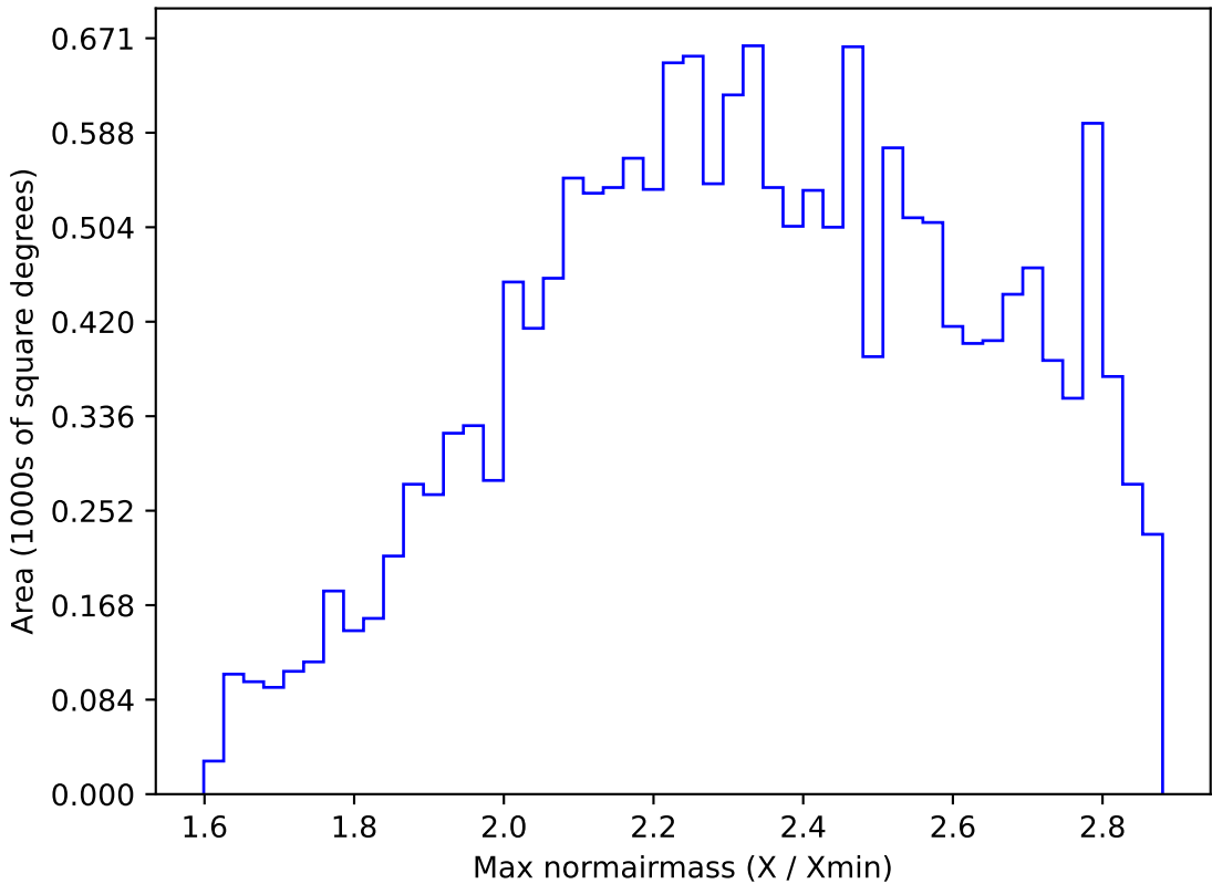
weather_cloudso8v3.4_10yrs WFD z band: Max normairmass
