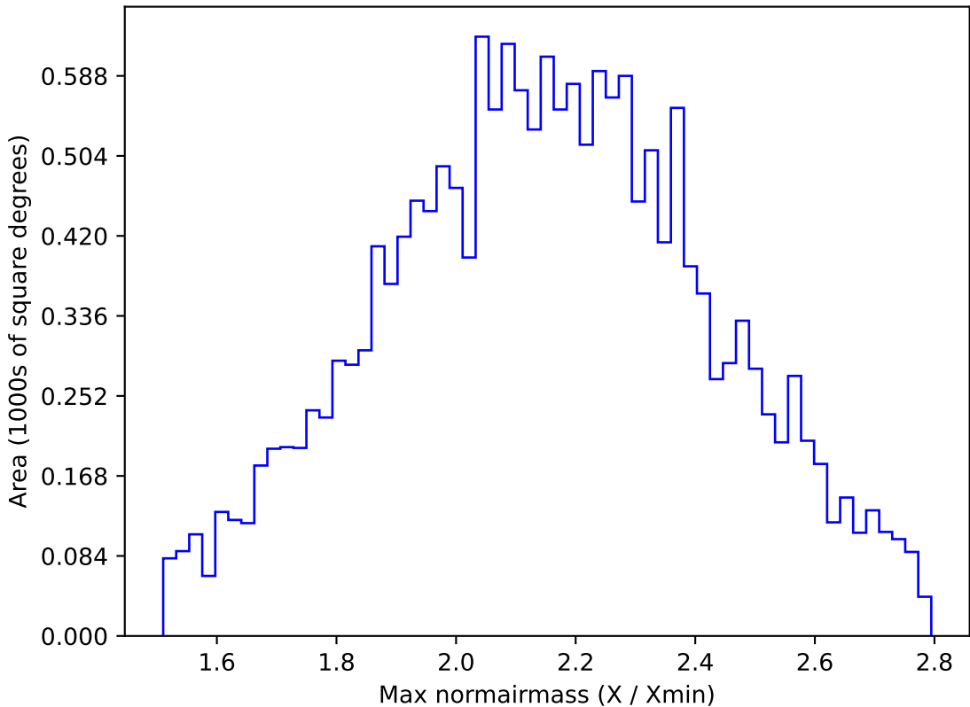
weather_cloudso8v3.4_10yrs WFD y band: Max normairmass
